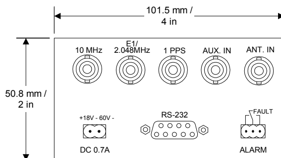
Example of connectors position (4531 GPS)
