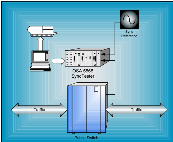
Figure 1: Typical application for the OSA 5565
