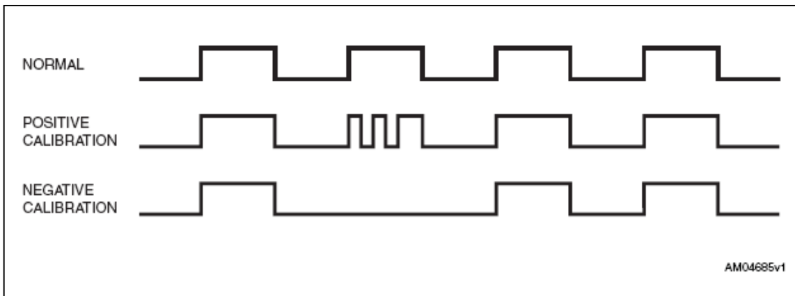
Figure 12. Calibration waveform
