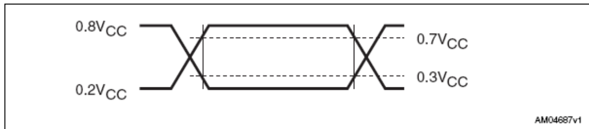
Figure 14. AC measurement I/O waveform
