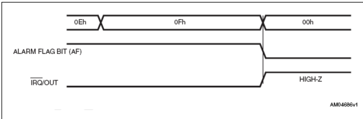
Figure 13. Alarm interrupt reset waveform
