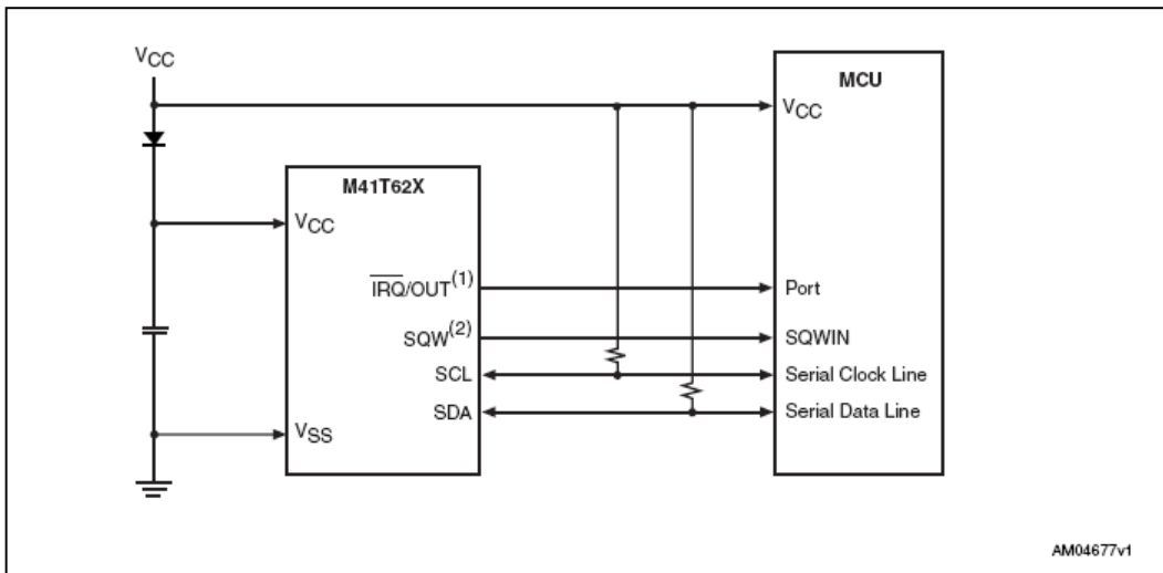
Figure 4. Hardware hookup for SuperCap™ backup operation
