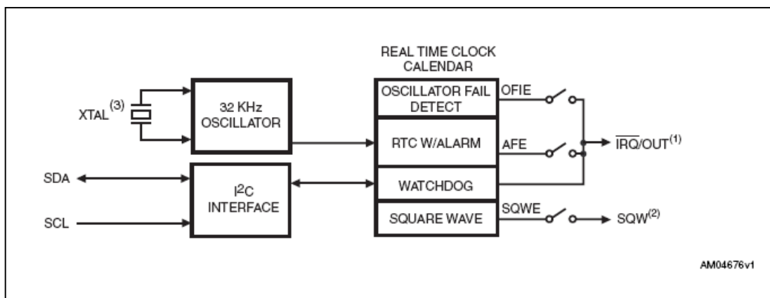
Figure 3. Block diagram
