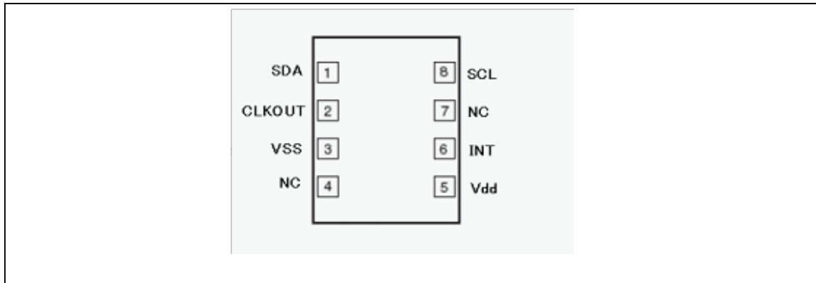
Figure 2. M41T62X connections
