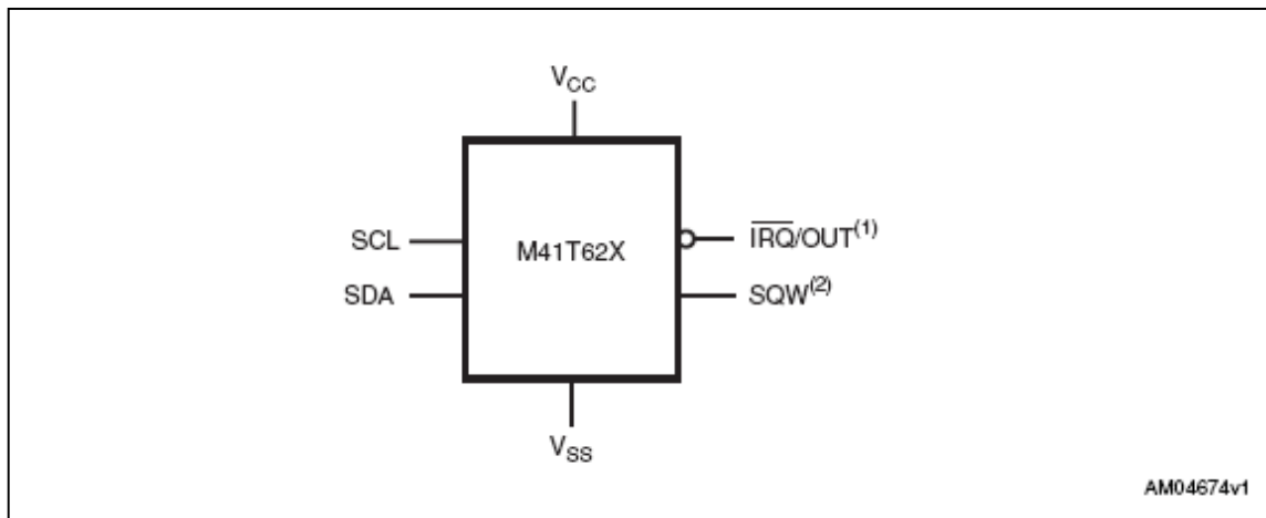
Figure 1. Logic diagram
