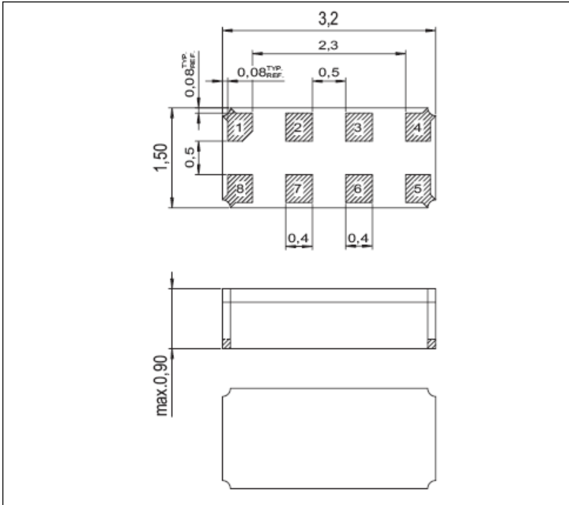
Figure 16. LCC – 8-pin 1.5 mm x 3.2 mm leadless chip carrier
