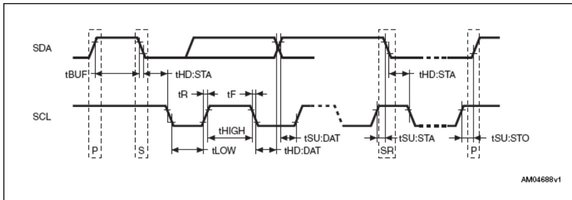
Figure 15. Bus timing requirements sequence
