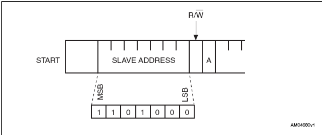
Figure 8. READ mode sequence
