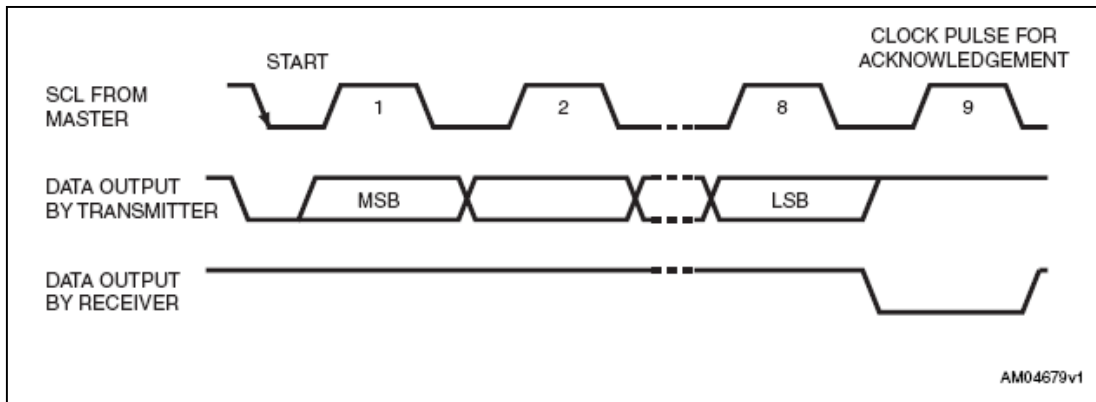
Figure 6. Acknowledgement sequence
