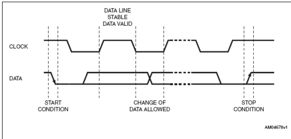
Figure 5. Serial bus data transfer sequence
